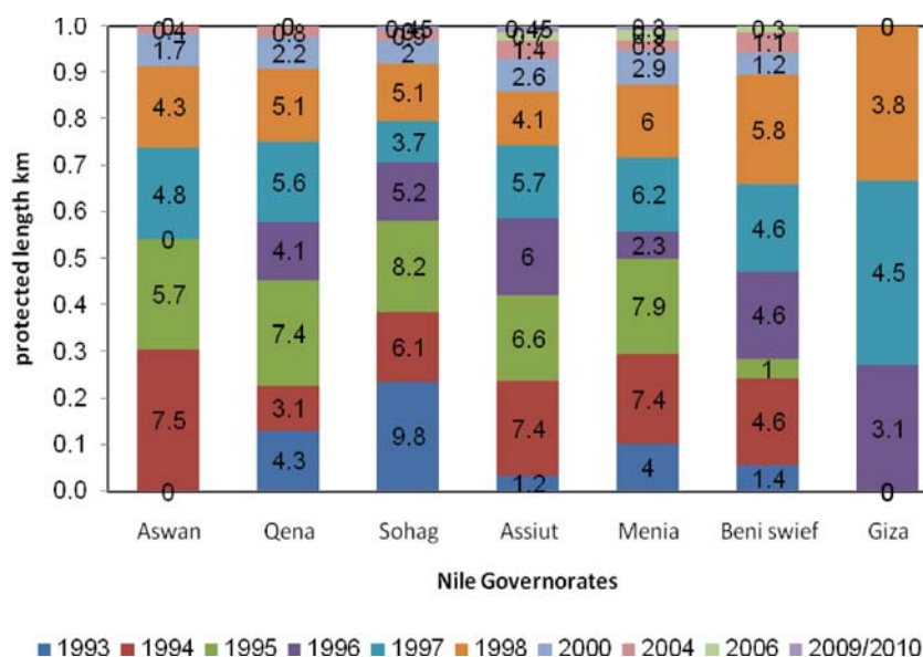
Fig. 8: Protection lengths distributed to Nile directorates
