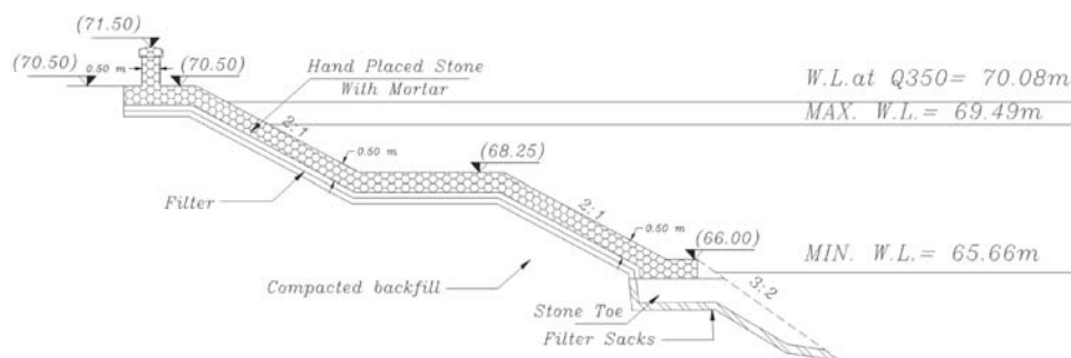
Fig. 7: Typical design for soil protection
