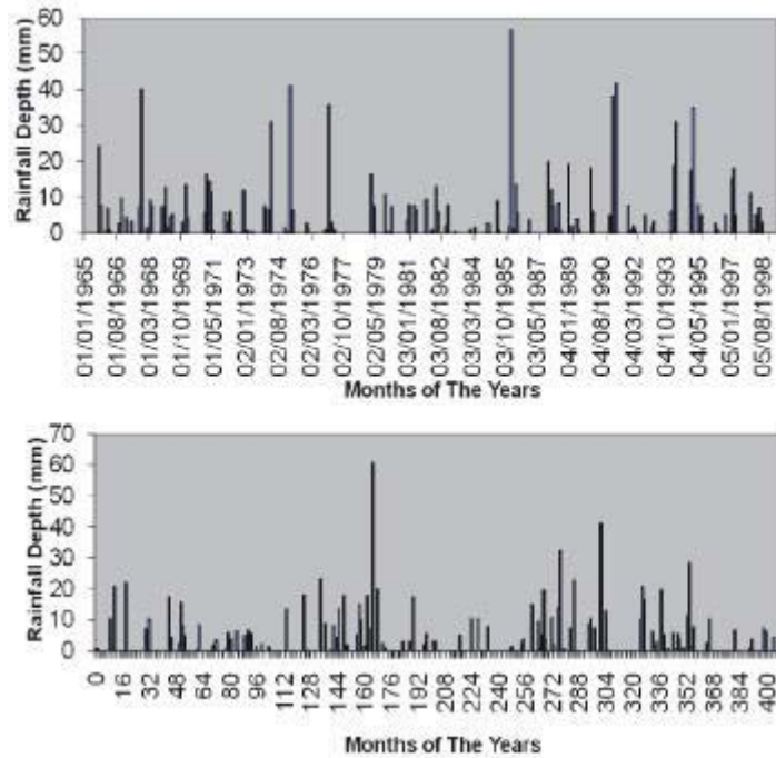
Fig. 7: Comparison between data (top) and simulation (bottom) of monthly rainfall depth at station Tabouk
