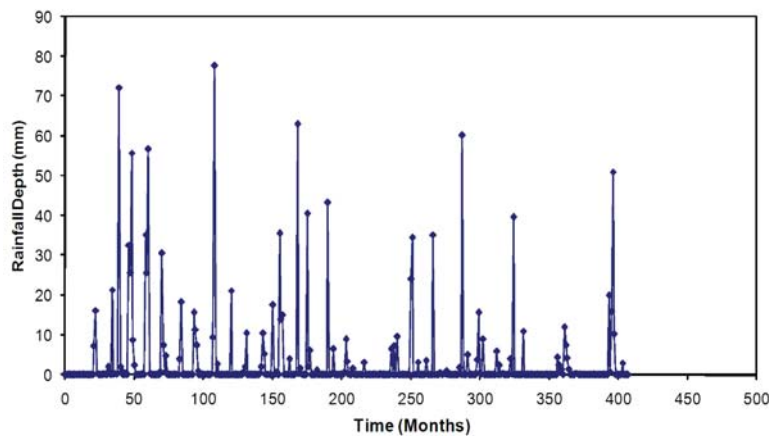
Fig. 1: A Typical monthly rainfall pattern at station J212 (records from 1965 to 1998)
