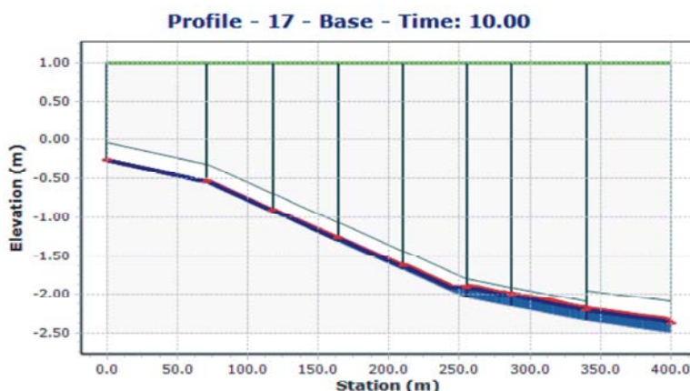
Fig. 2: Longitudinal profile in the sewer pipeline from segment CO-19 to segment CO-10 at time 10 AM.
