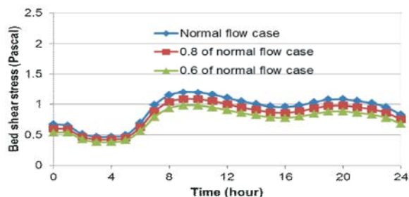
Fig. 5: Time variation of bed shear stress in pipe CO-2 for normal flow, 0.8 of normal flow and 0.6 of normal flow cases.
